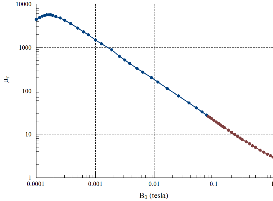
Figure 30: Extension of the saturation curve for 50H470 steel. Blue points are experimental values while red points represent the analytic extrapolation.
