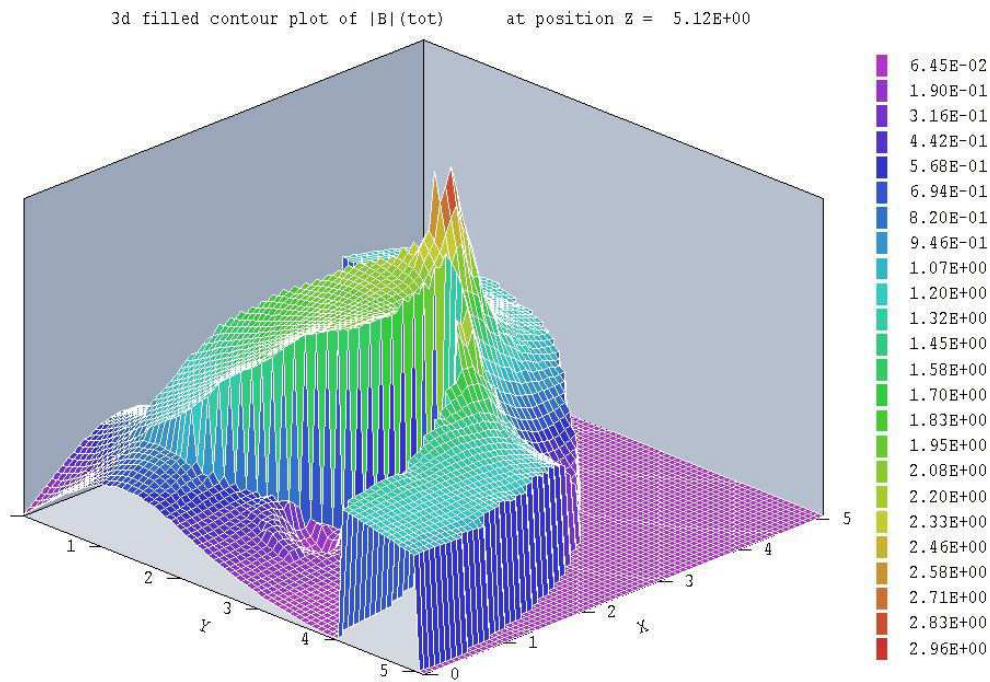
Figure 40: Plane plot of |B| – type 3D filled contour .
