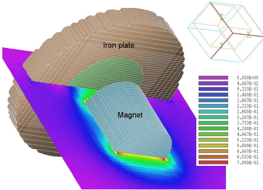
Figure 57: Geometry for the PMAGFORCE example.
