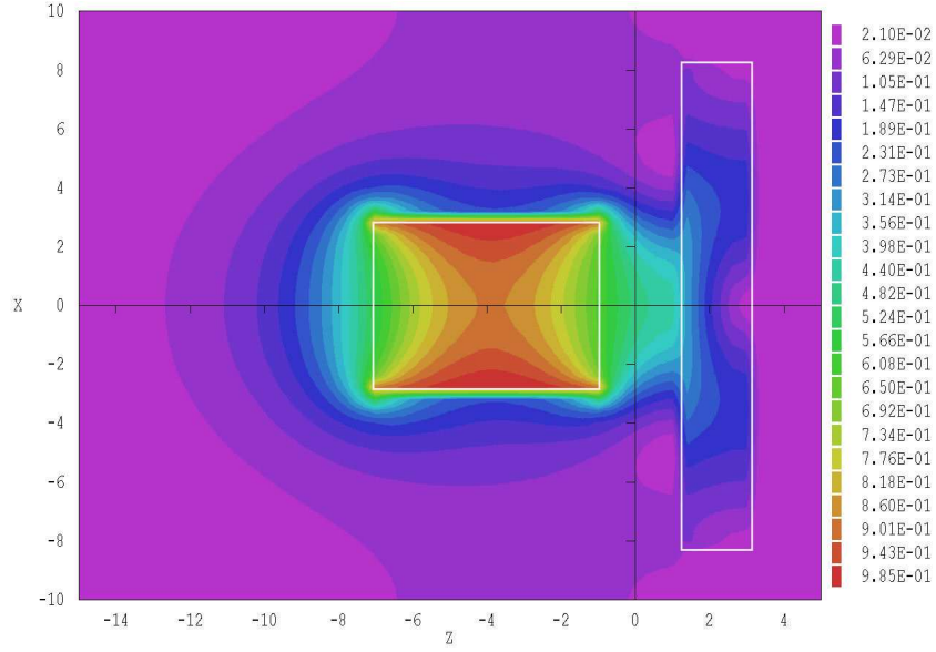
Figure 58: Example PMAGFORCE, variation of |\mathbf{B}| in the plane y = 0.0 .
