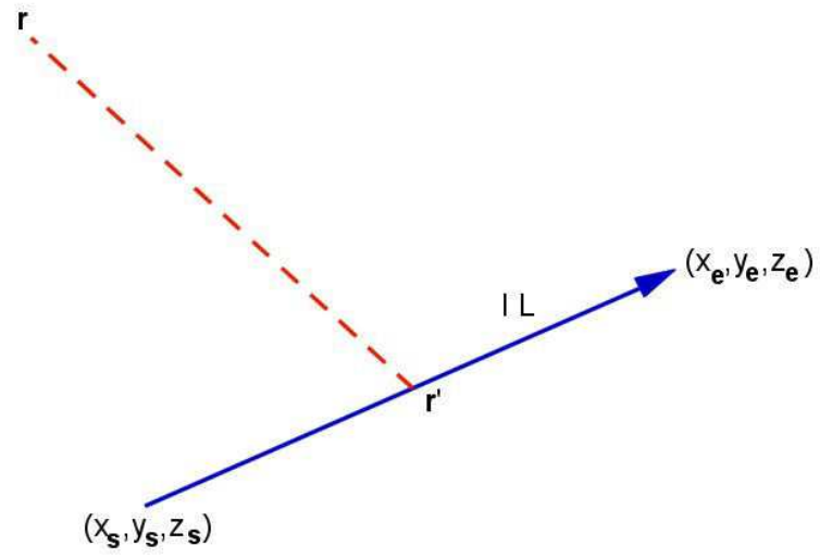
Figure 8: Current-element geometry.
