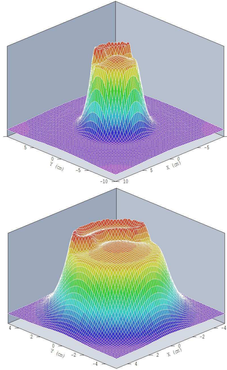
Figure 35: Plot of |\mathbf{B}| in the plane z = 1.1 \text{ cm} . Top: macroscopic solution. Bottom: microscopic solution. The peak field value is 1.9 tesla.
