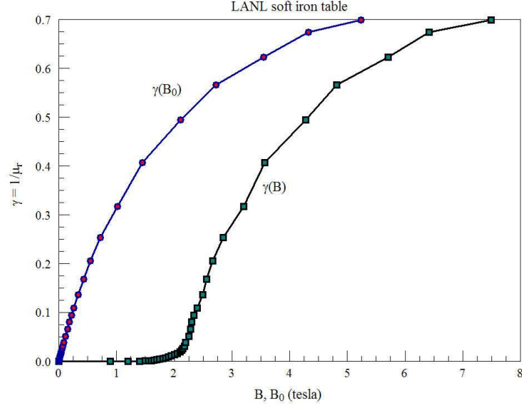
Figure 29: The parameter \gamma = 1/\mu_r for soft iron as a function of |\mathbf{B}| (green squares) and |\mathbf{B}_0| (red circles). Adapted from the Superfish/Poisson Manual, Los Alamos National Laboratory.
