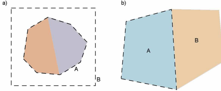
Figure 56: Surface integral of the magnetic stress tensor. a) Valid surfaces for an integral of magnetically-active materials. A: region surfaces bounded by air elements. B: surface of an air region that encloses the magnetic materials. b) Invalid surface for an integral. The enclosed material current is undefined on the common boundary.
