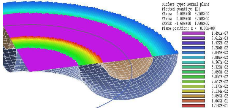
Figure 12: Example SURFCURRENT – |\mathbf{B}| in the plane z = 0.0 .
