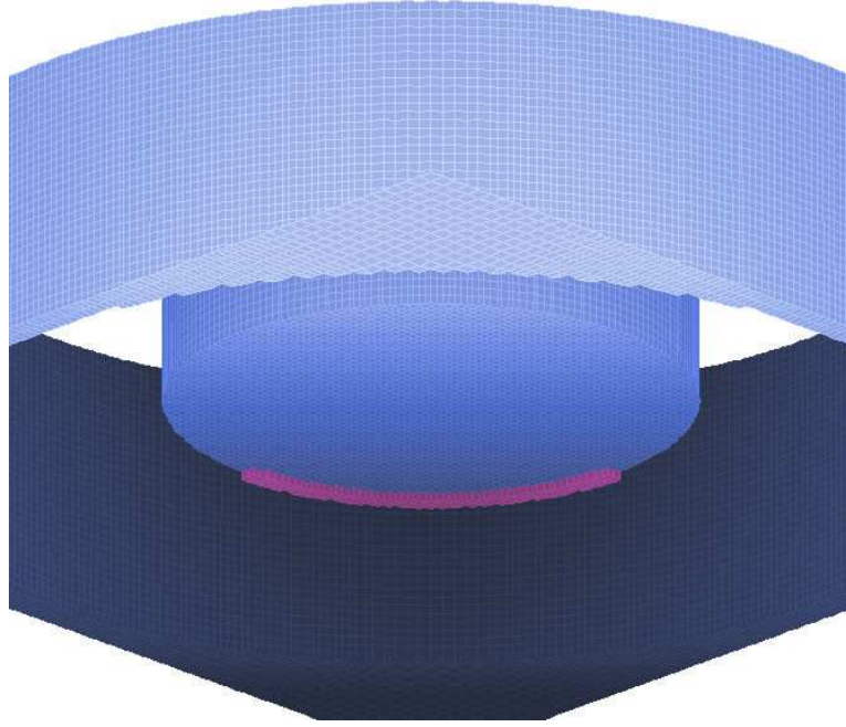
Figure 26: Example MAGNUMBOUND : three-dimensional view of the upper pole face in the microscopic solution showing the pole extension (violet).
