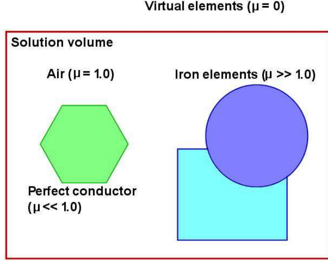
Figure 13: Schematic view - division of the solution volume for a dual-potential solution.
