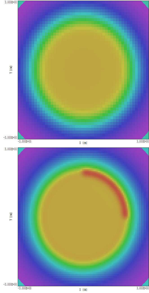
Figure 27: Example MAGNUMBOUND : details of the variation of |\mathbf{B}| in the x - y plane at z = 0.281 cm. Values range: 0.0 tesla (violet), 1.35 tesla (red). Top: macroscopic solution. Bottom: microscopic solution with pole extension.
