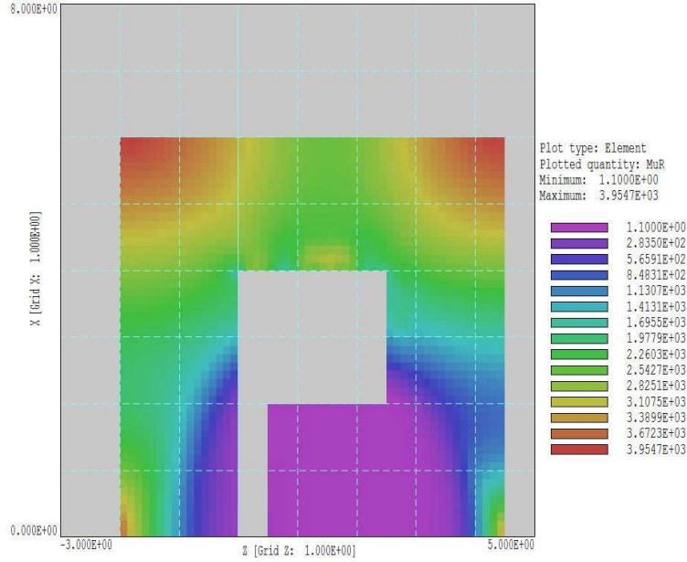
Figure 33: Spatial distribution of \mu_r for the final Magnum solution in the plane y = 0.0 .
