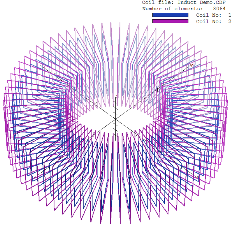
Figure 60: Primary and secondary windings created with MagWinder for the InductDemo example.
