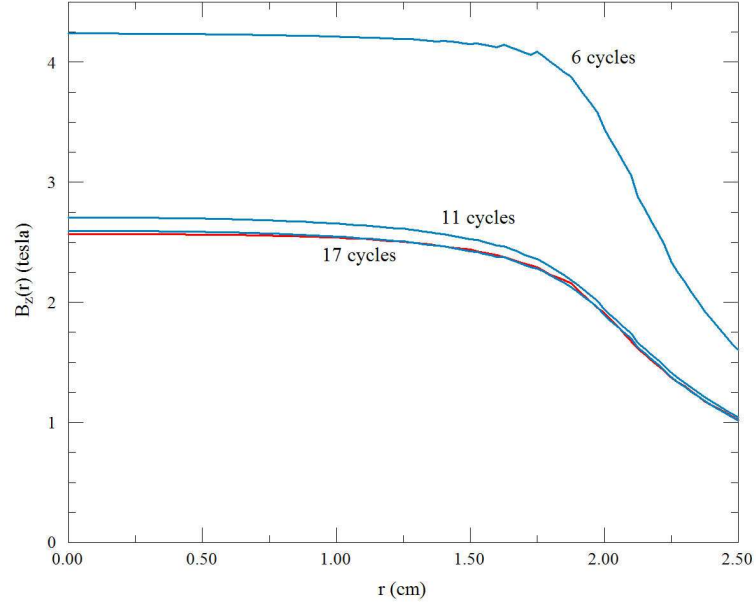
Figure 32: Radial scans of B_z at z = 0.25 cm. Red line: PerMag solution. Blue lines: Magnum solutions with different values of NCycle .
