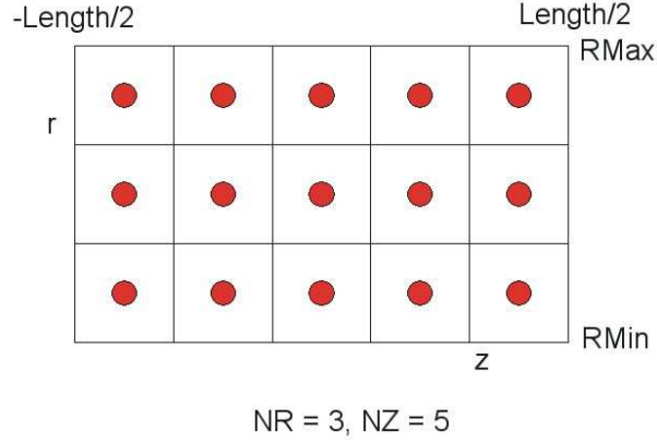
Figure 20: Arrangement of wires in the SOLENOID model.
