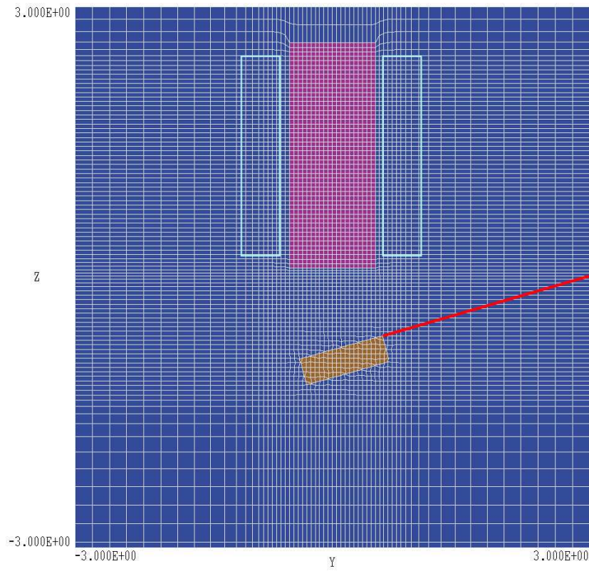
Figure 59: Geometry and mesh for example RELAY (view in the plane x = 0.0 ). Violet region: iron core. Light-blue outline: solenoid coil. Orange region: iron plate attached to structure (red line) hinged along an axis parallel to x at y = 3.0, z = 0.0 .
