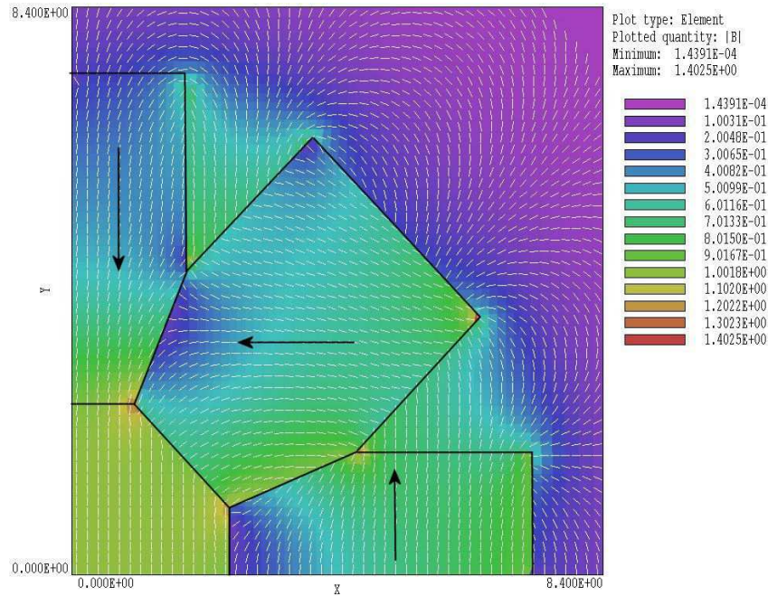
Figure 24: Magnum calculation of a permanent-magnet ring dipole (single quadrant with symmetry boundaries). Vector lines with color-coding by |\mathbf{B}| . Black arrows show magnetization vectors.
