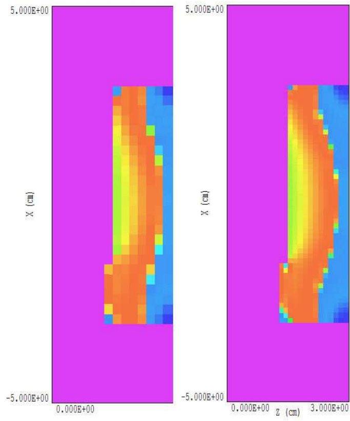
Figure 36: Plot of \mu_r in the plane y = 0.0 . Left: portion of the macroscopic solution. Right: full extent of the microscopic solution. Violet: \mu_r = 1.0 , red: \mu_r = 6.0
